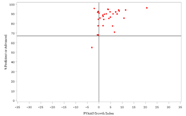
2011 PSSA % Proficient or Advanced vs PVAAS Growth Index Test=PSSA End-of-Grade Subject=Math Grade=7
