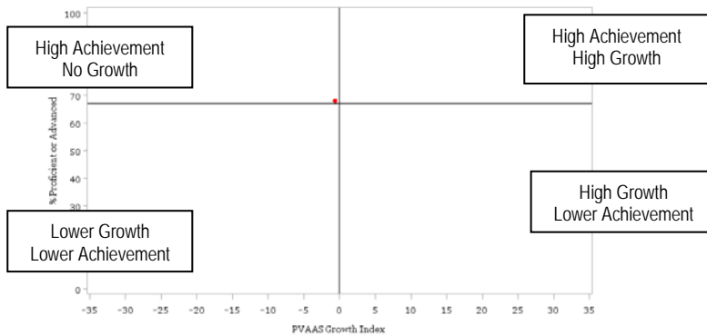
2011 PSSA % Proficient or Advanced vs PVAAS Growth Index Test=PSSA End-of-Grade Subject=Math Grade=7
