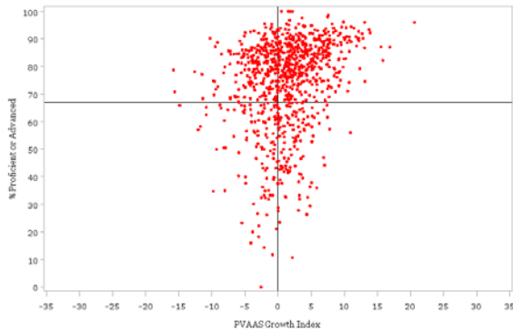
2011 State-wide PSSA % Proficient or Advanced vs PVAAS Growth Index Test=PSSA End-of-Grade Subject=Math Grade=7
